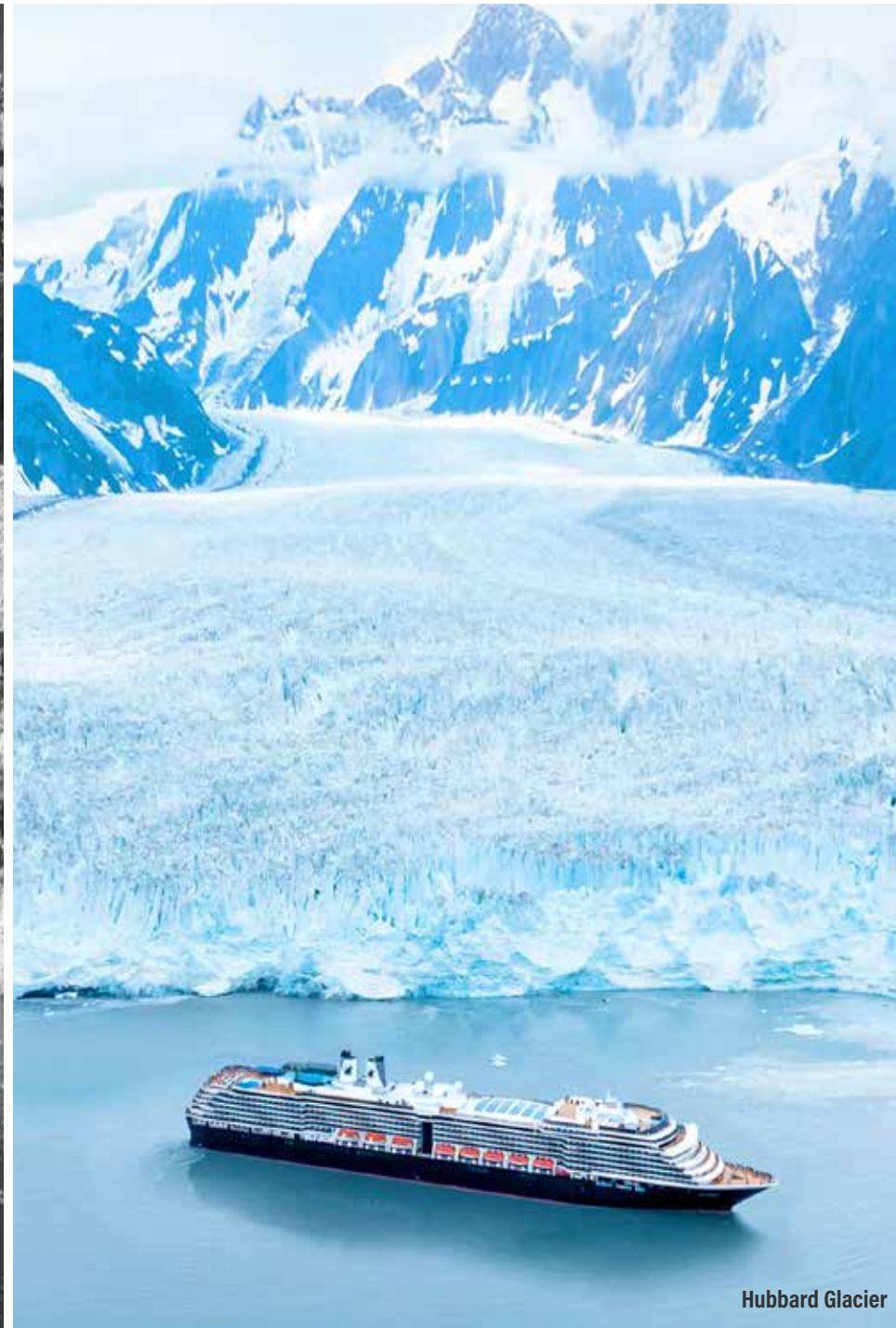
Hubbard Glacier
